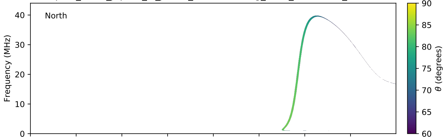
expres_earth_jupiter_io_jrm09_lossc-wid1deg_3kev_20050503_v01.cdf
