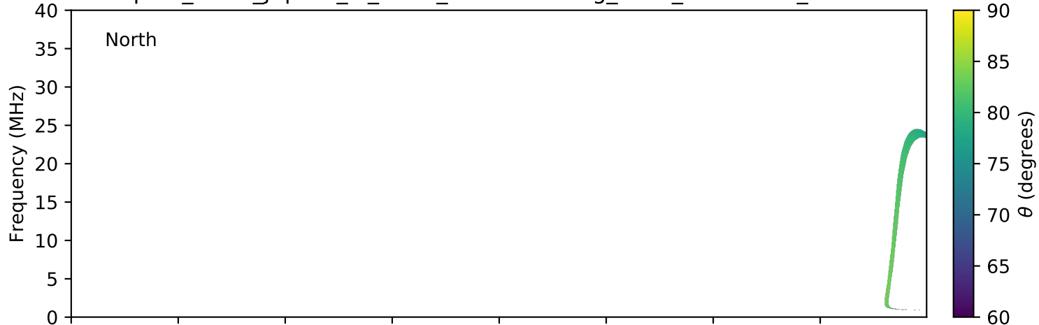
expres_earth_jupiter_io_isaac_lossc-wid1deg_3kev_20050531_v01.cdf
