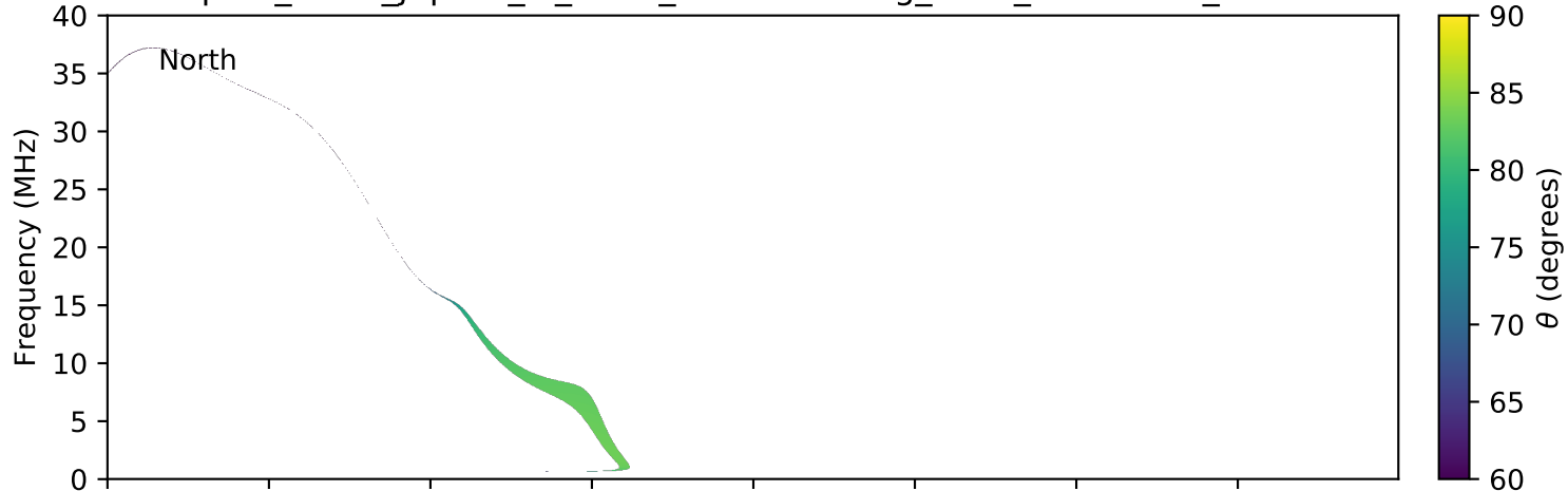
expres_earth_jupiter_io_isaac_lossc-wid1deg_3kev_20050527_v01.cdf
