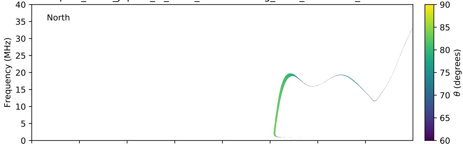
expres_earth_jupiter_io_isaac_lossc-wid1deg_3kev_20050526_v01.cdf
