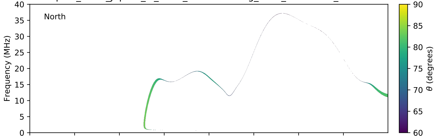
expres_earth_jupiter_io_isaac_lossc-wid1deg_3kev_20050521_v01.cdf
