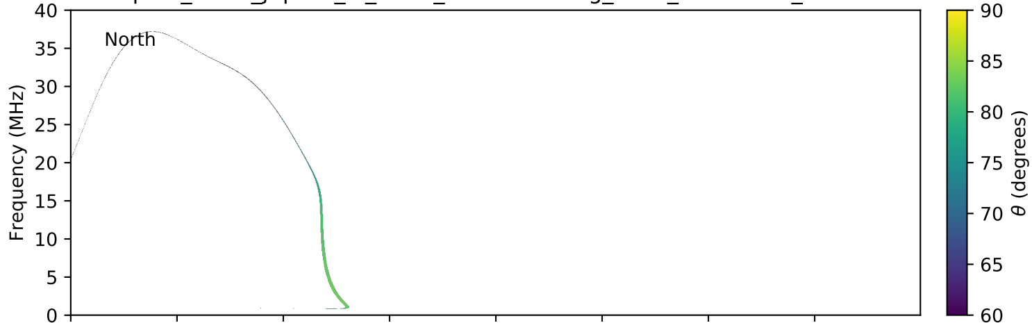
expres_earth_jupiter_io_isaac_lossc-wid1deg_3kev_20050520_v01.cdf
