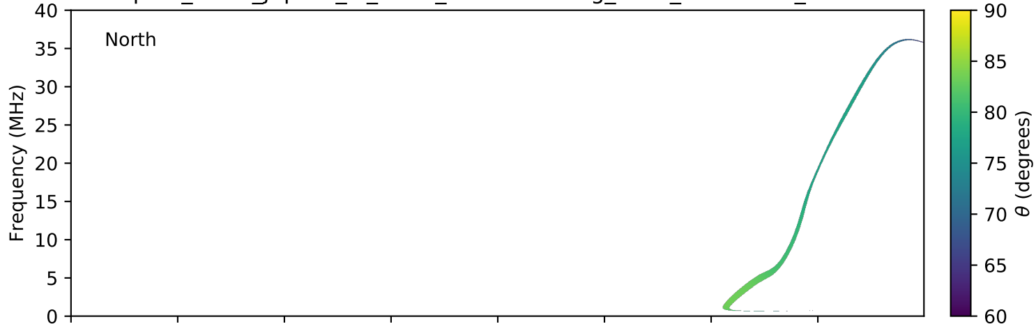
expres_earth_jupiter_io_isaac_lossc-wid1deg_3kev_20050517_v01.cdf
