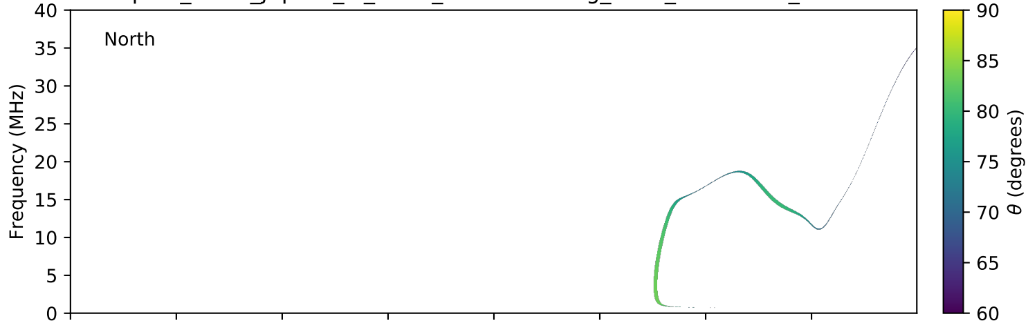
expres_earth_jupiter_io_isaac_lossc-wid1deg_3kev_20050510_v01.cdf
