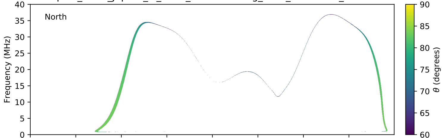
expres_earth_jupiter_io_isaac_lossc-wid1deg_3kev_20050507_v01.cdf
