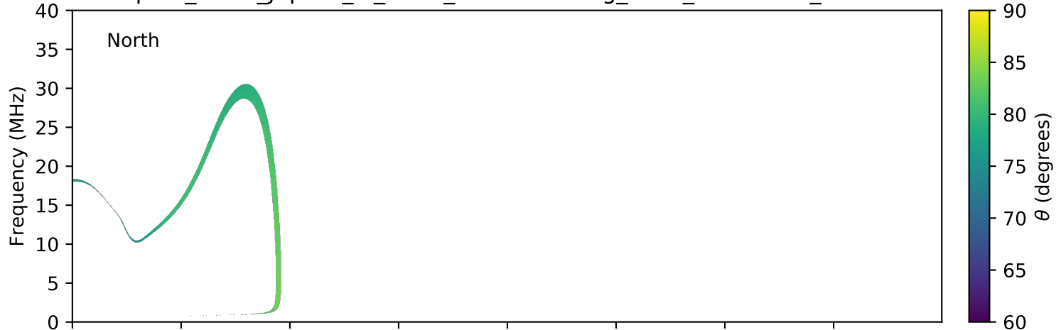
expres_earth_jupiter_io_isaac_lossc-wid1deg_3kev_20050506_v01.cdf
