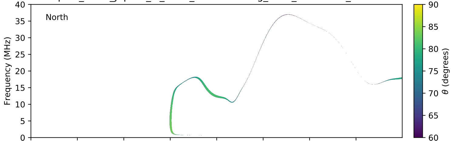
expres_earth_jupiter_io_isaac_lossc-wid1deg_3kev_20050505_v01.cdf
