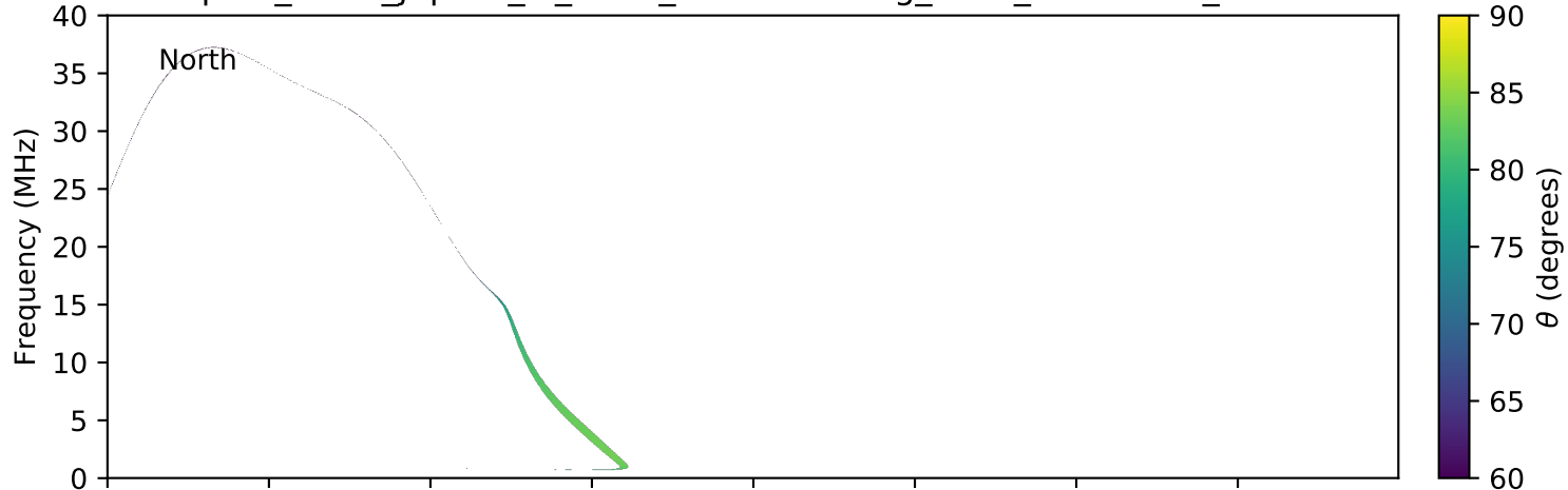
expres_earth_jupiter_io_isaac_lossc-wid1deg_3kev_20050504_v01.cdf
