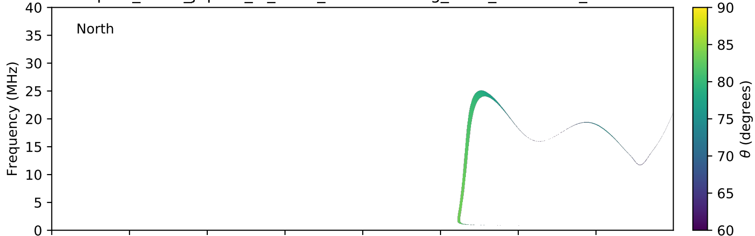
expres_earth_jupiter_io_isaac_lossc-wid1deg_3kev_20050503_v01.cdf
