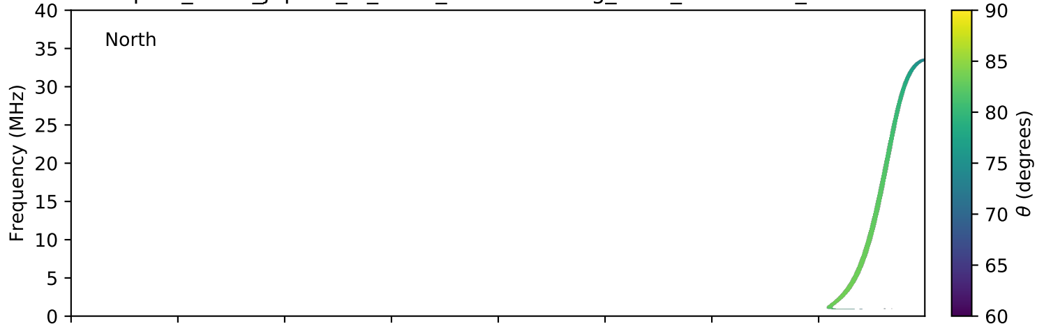
expres_earth_jupiter_io_isaac_lossc-wid1deg_3kev_20050501_v01.cdf
