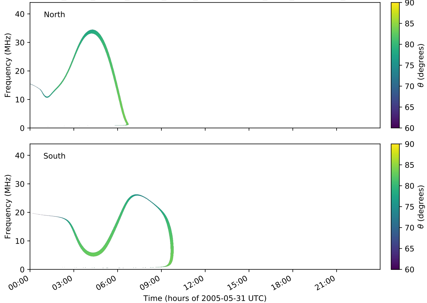
expres_earth_jupiter_europa_jrm09_lossc-wid1deg_3kev_20050531_v01.cdf
