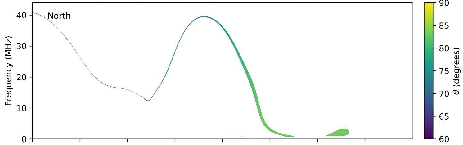
expres_earth_jupiter_europa_jrm09_lossc-wid1deg_3kev_20050527_v01.cdf
