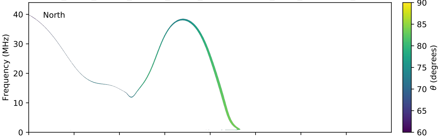
expres_earth_jupiter_europa_jrm09_lossc-wid1deg_3kev_20050520_v01.cdf
