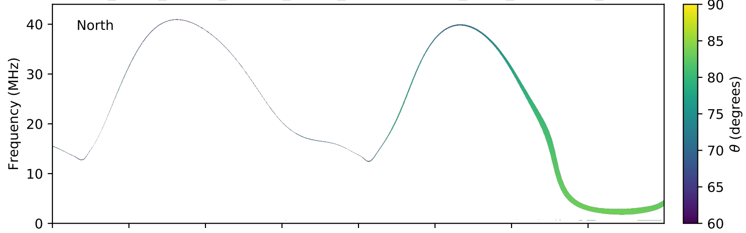
expres_earth_jupiter_europa_jrm09_lossc-wid1deg_3kev_20050509_v01.cdf
