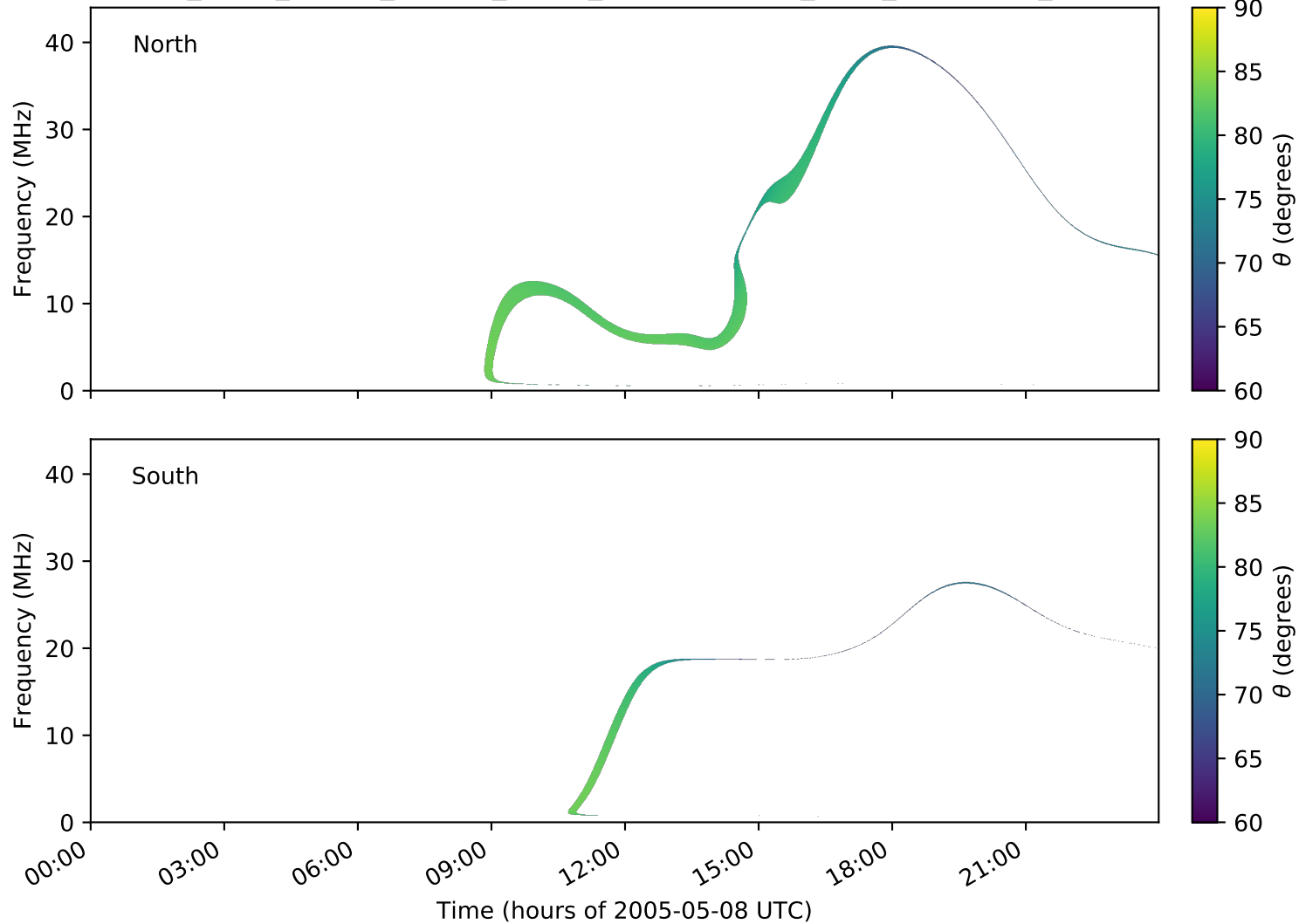
expres_earth_jupiter_europa_jrm09_lossc-wid1deg_3kev_20050508_v01.cdf
