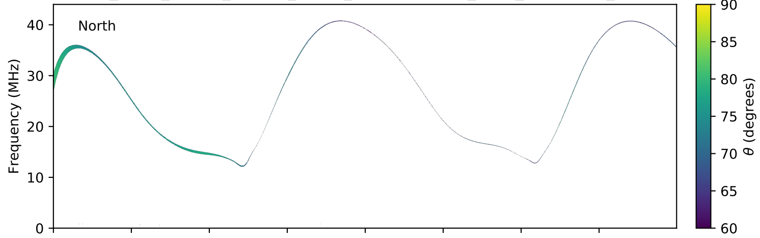
expres_earth_jupiter_europa_jrm09_lossc-wid1deg_3kev_20050505_v01.cdf
