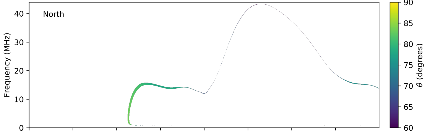
expres_earth_jupiter_io_jrm09_lossc-wid1deg_3kev_20050329_v01.cdf
