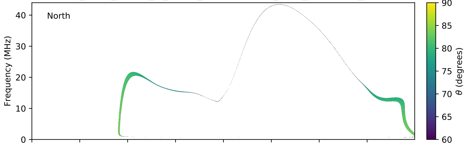
expres_earth_jupiter_io_jrm09_lossc-wid1deg_3kev_20050322_v01.cdf
