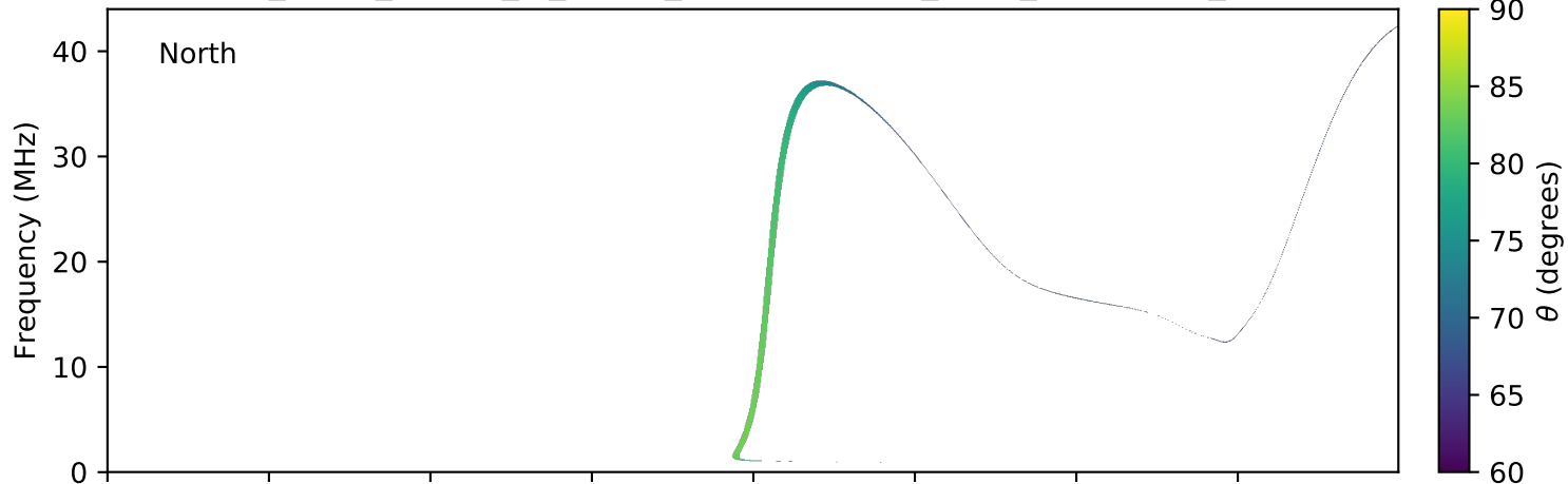
expres_earth_jupiter_io_jrm09_lossc-wid1deg_3kev_20050320_v01.cdf
