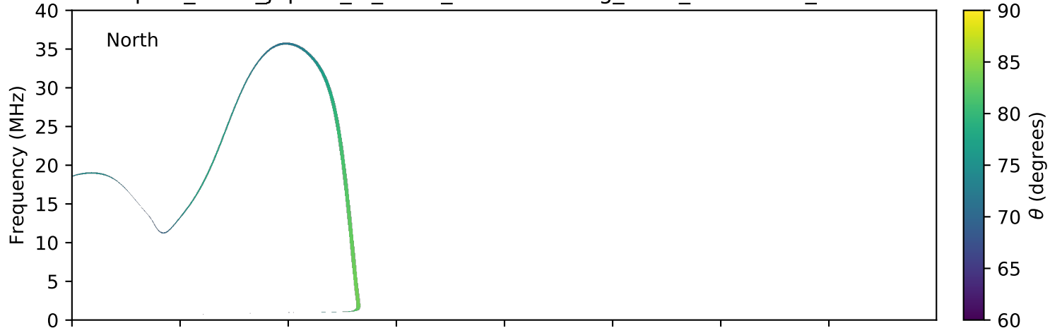
expres_earth_jupiter_io_isaac_lossc-wid1deg_3kev_20050328_v01.cdf
