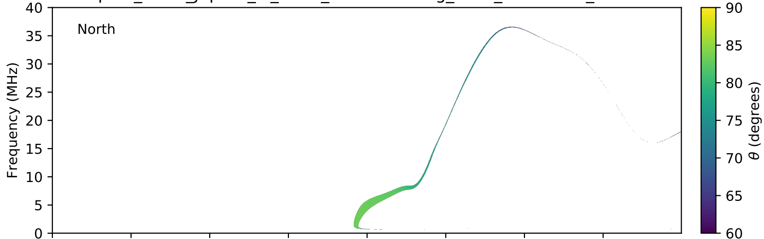
expres_earth_jupiter_io_isaac_lossc-wid1deg_3kev_20050327_v01.cdf
