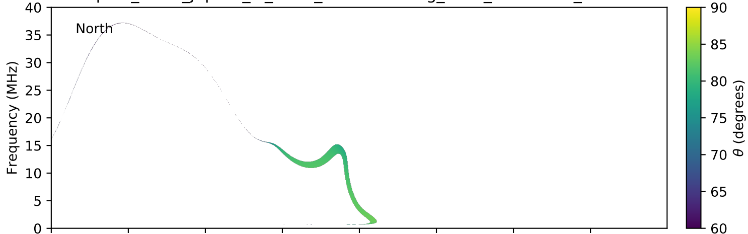
expres_earth_jupiter_io_isaac_lossc-wid1deg_3kev_20050326_v01.cdf
