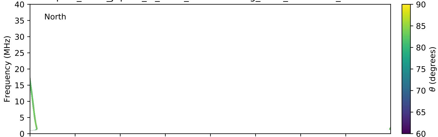
expres_earth_jupiter_io_isaac_lossc-wid1deg_3kev_20050323_v01.cdf
