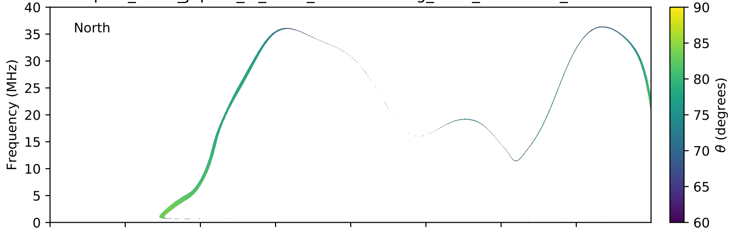
expres_earth_jupiter_io_isaac_lossc-wid1deg_3kev_20050322_v01.cdf
