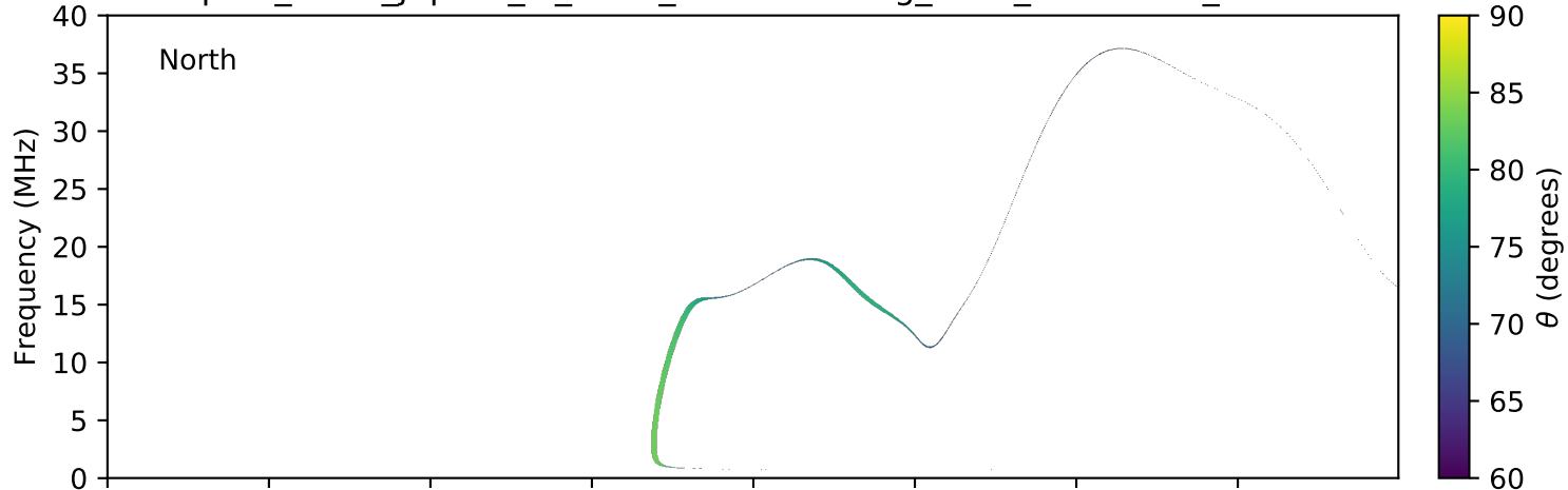
expres_earth_jupiter_io_isaac_lossc-wid1deg_3kev_20050320_v01.cdf
