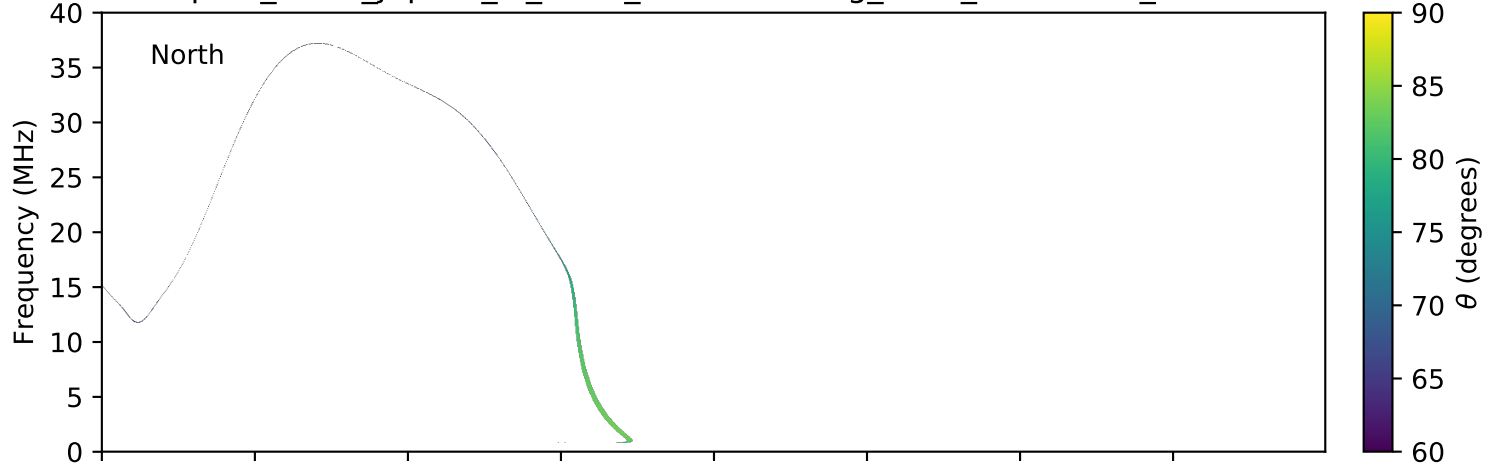
expres_earth_jupiter_io_isaac_lossc-wid1deg_3kev_20050319_v01.cdf
