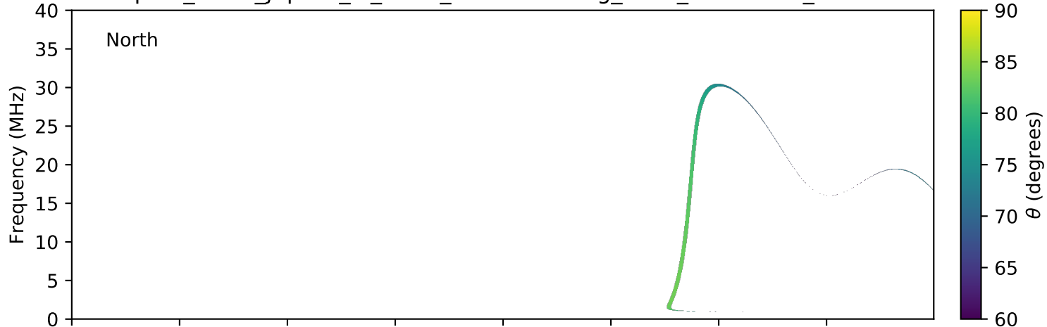
expres_earth_jupiter_io_isaac_lossc-wid1deg_3kev_20050318_v01.cdf
