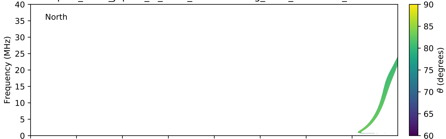
expres_earth_jupiter_io_isaac_lossc-wid1deg_3kev_20050316_v01.cdf
