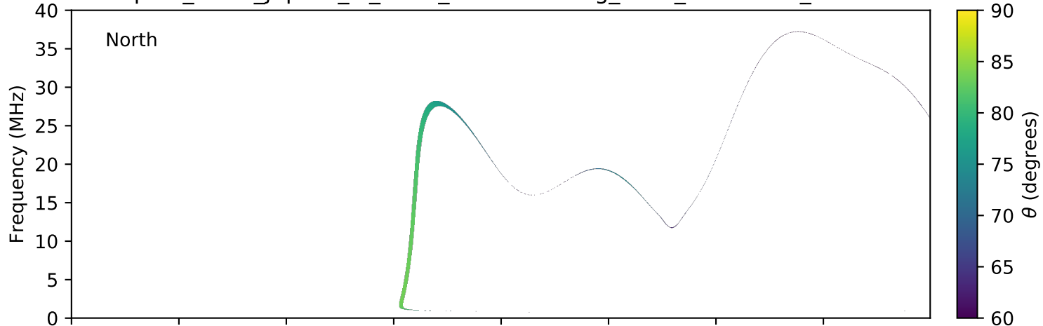
expres_earth_jupiter_io_isaac_lossc-wid1deg_3kev_20050313_v01.cdf
