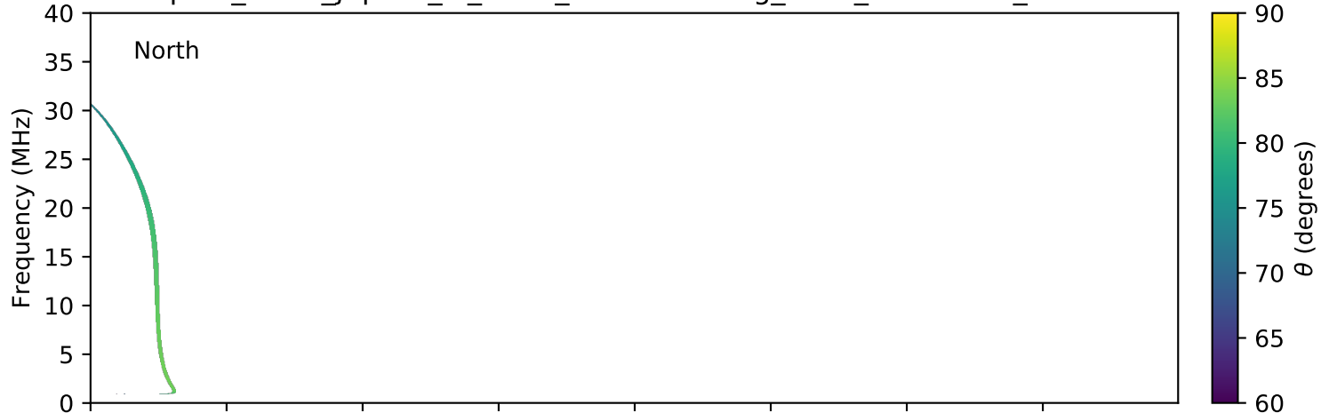
expres_earth_jupiter_io_isaac_lossc-wid1deg_3kev_20050307_v01.cdf
