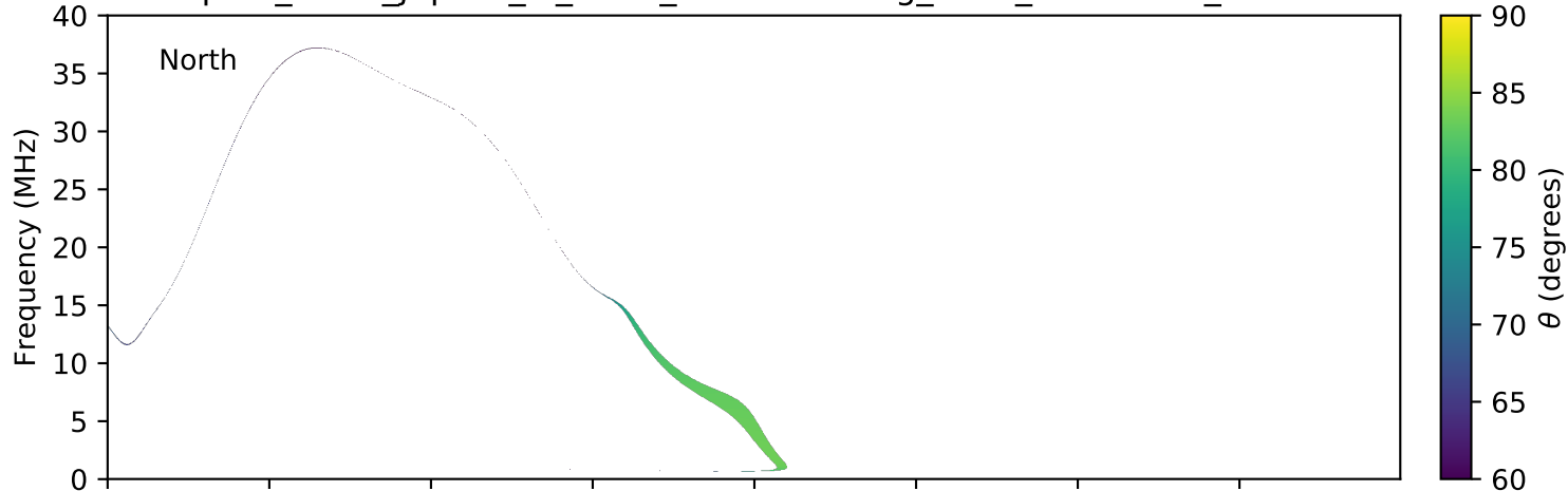
expres_earth_jupiter_io_isaac_lossc-wid1deg_3kev_20050303_v01.cdf
