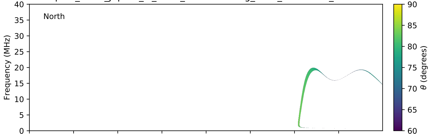
expres_earth_jupiter_io_isaac_lossc-wid1deg_3kev_20050302_v01.cdf
