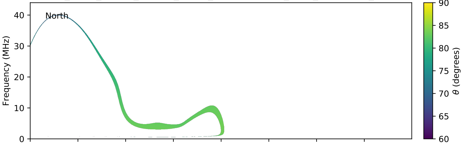
expres_earth_jupiter_europa_jrm09_lossc-wid1deg_3kev_20050328_v01.cdf
