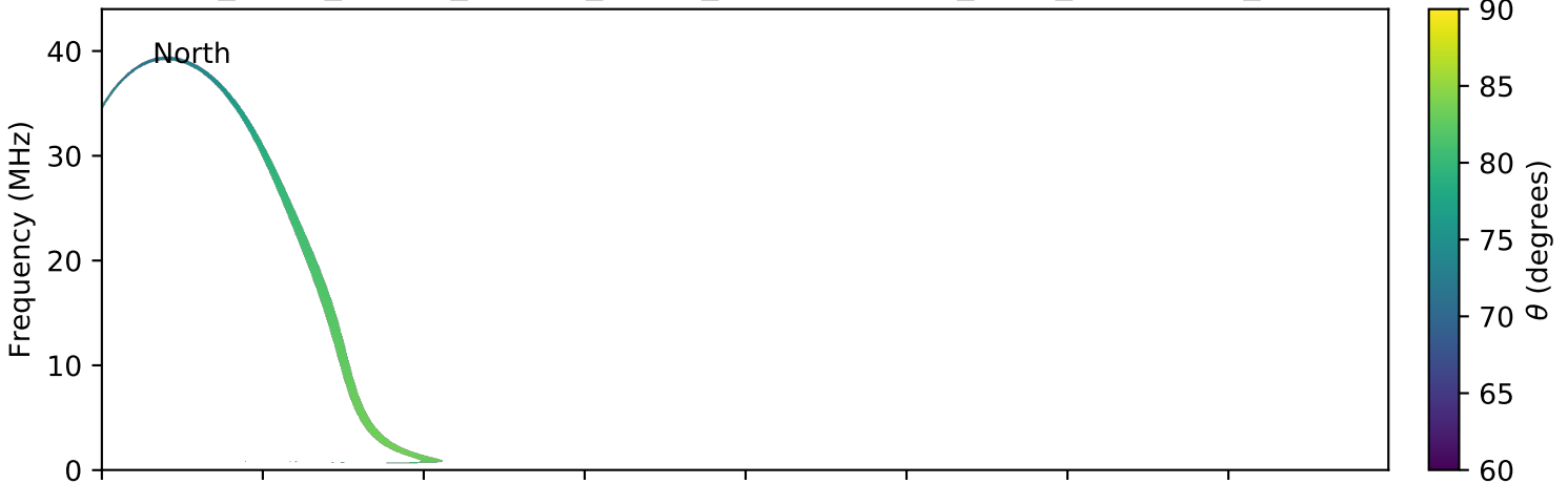
expres_earth_jupiter_europa_jrm09_lossc-wid1deg_3kev_20050321_v01.cdf
