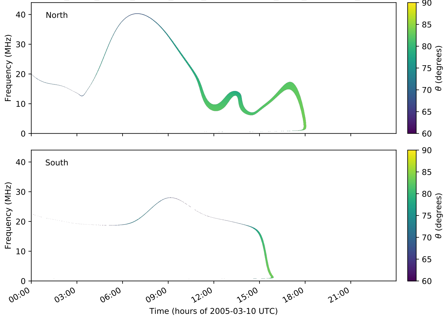
expres_earth_jupiter_europa_jrm09_lossc-wid1deg_3kev_20050310_v01.cdf
