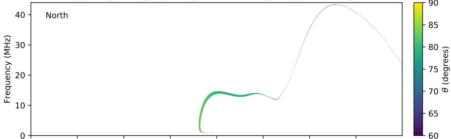
expres_earth_jupiter_io_jrm09_lossc-wid1deg_3kev_20050225_v01.cdf
