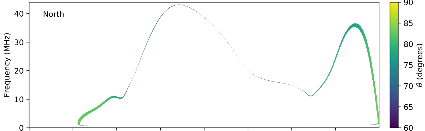
expres_earth_jupiter_io_jrm09_lossc-wid1deg_3kev_20050220_v01.cdf
