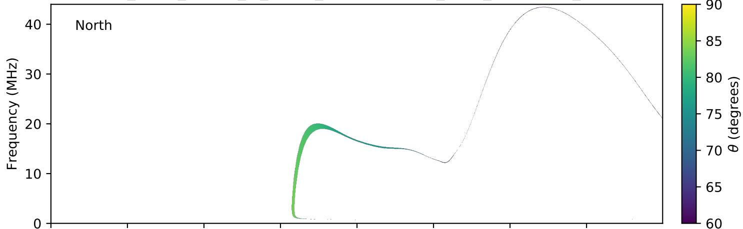
expres_earth_jupiter_io_jrm09_lossc-wid1deg_3kev_20050218_v01.cdf
