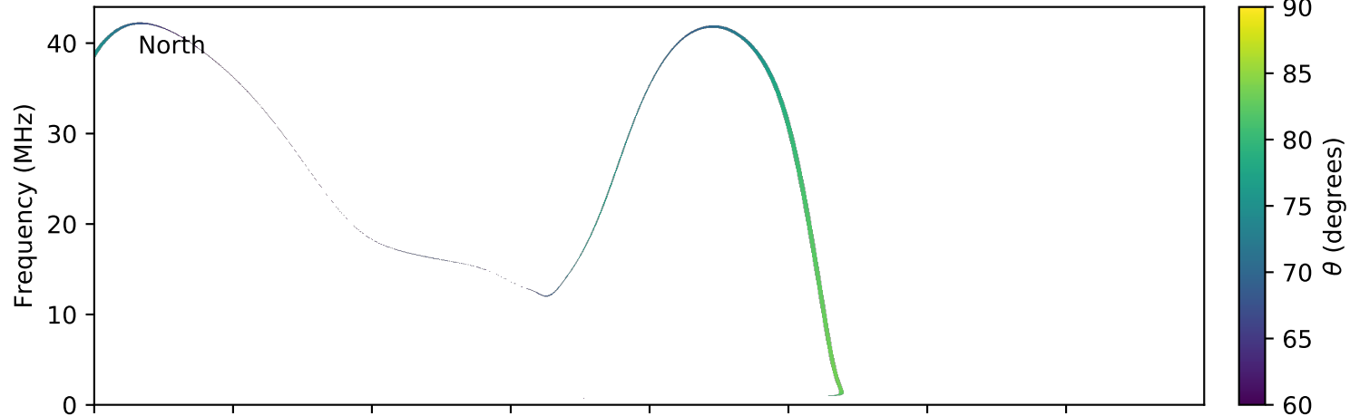
expres_earth_jupiter_io_jrm09_lossc-wid1deg_3kev_20050215_v01.cdf
