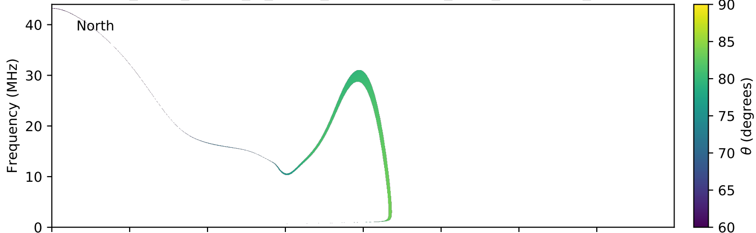
expres_earth_jupiter_io_jrm09_lossc-wid1deg_3kev_20050201_v01.cdf
