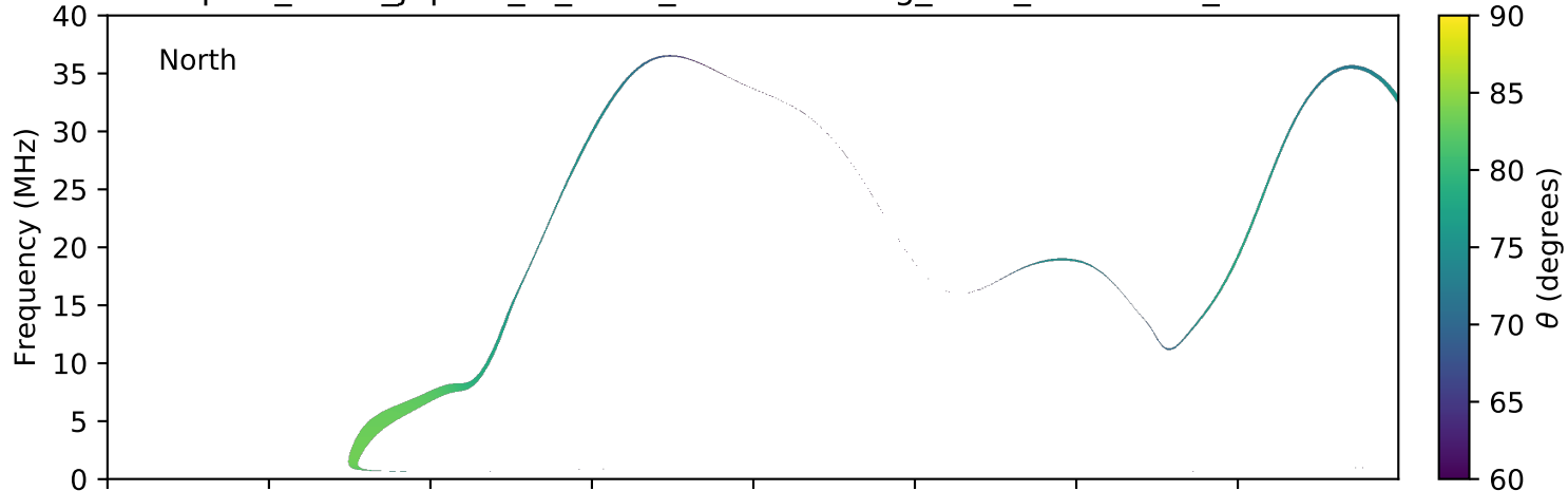
expres_earth_jupiter_io_isaac_lossc-wid1deg_3kev_20050227_v01.cdf
