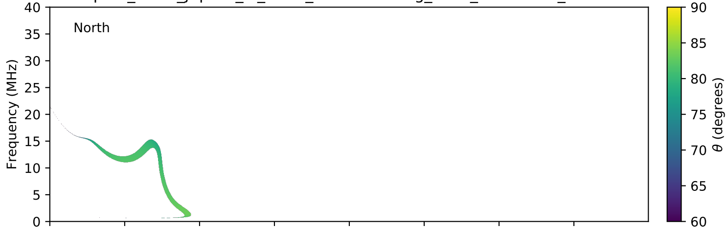
expres_earth_jupiter_io_isaac_lossc-wid1deg_3kev_20050226_v01.cdf
