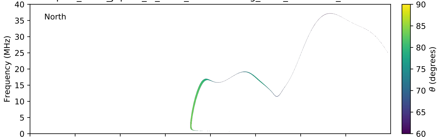
expres_earth_jupiter_io_isaac_lossc-wid1deg_3kev_20050225_v01.cdf
