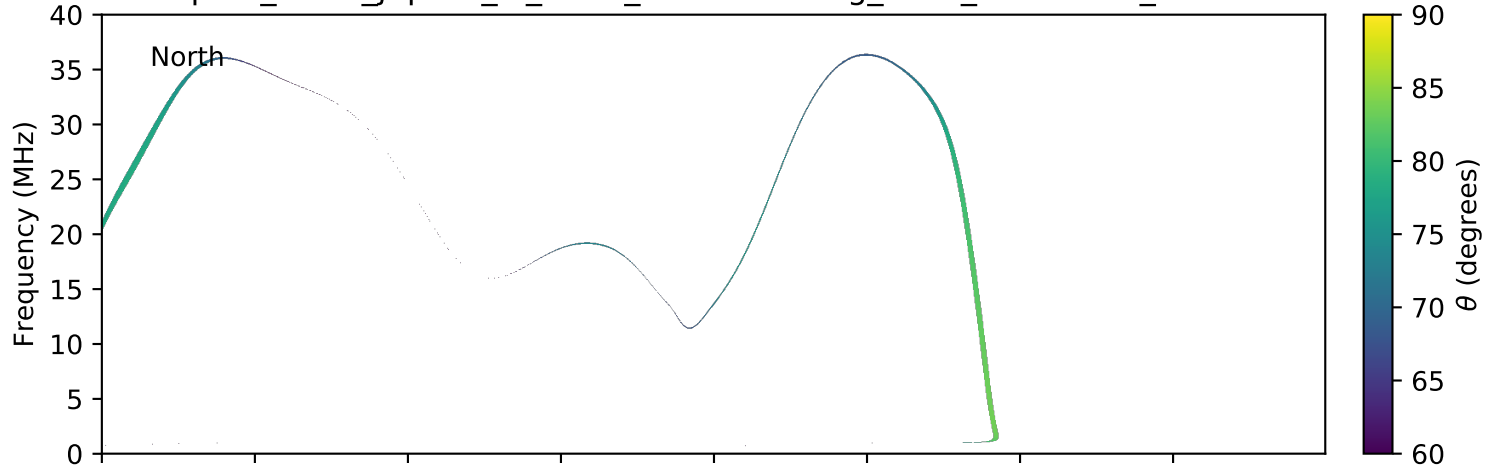
expres_earth_jupiter_io_isaac_lossc-wid1deg_3kev_20050222_v01.cdf
