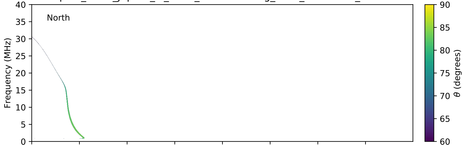
expres_earth_jupiter_io_isaac_lossc-wid1deg_3kev_20050219_v01.cdf
