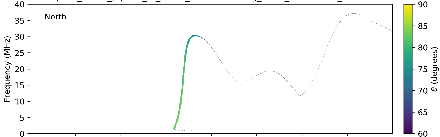
expres_earth_jupiter_io_isaac_lossc-wid1deg_3kev_20050218_v01.cdf
